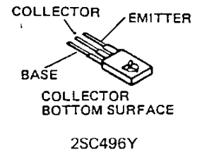
Viewed from component side
